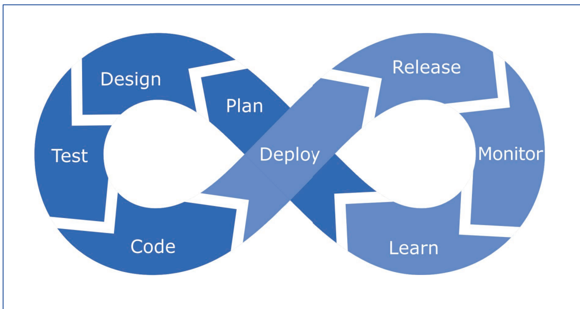
Figure 1-1, DevOps Lemniscate.
